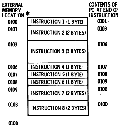
Fig. 2-7. Program counter operation.
