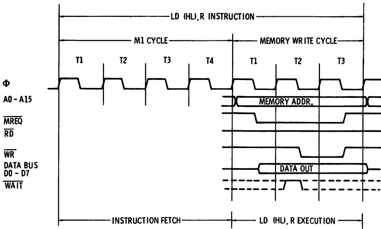
Fig. 3-5. Write cycle.
