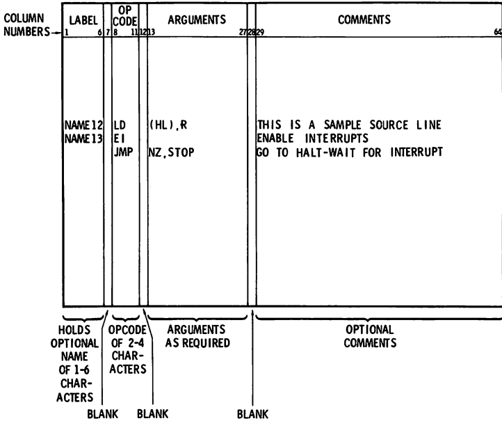
Fig. 9-3. Typical Z-80 assembly language format.
