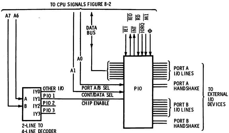
Fig. 8-12. PIO use in minimum configuration system.
