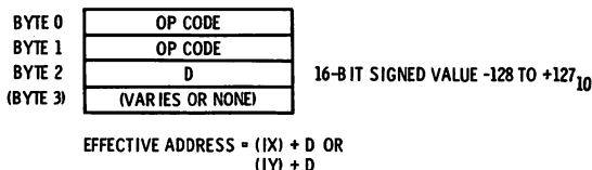
Fig. 4-17. Indexed addressing.
