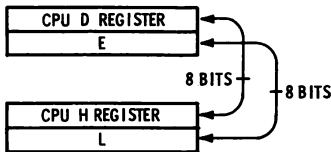
Fig. 5-3. EX DE, HL instructions.
