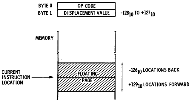
Fig. 4-15. Relative addressing.
