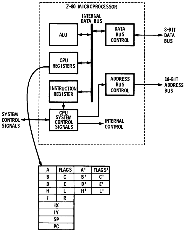
Fig. 2-1. Z-80 Microprocessor architecture.
