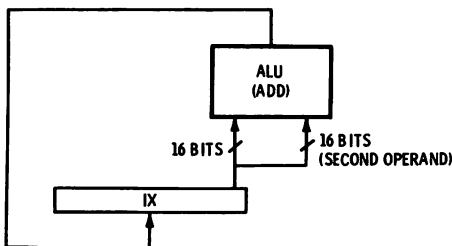
Fig. 5-14. Sixteen-bit arithmetic instruction examples.
