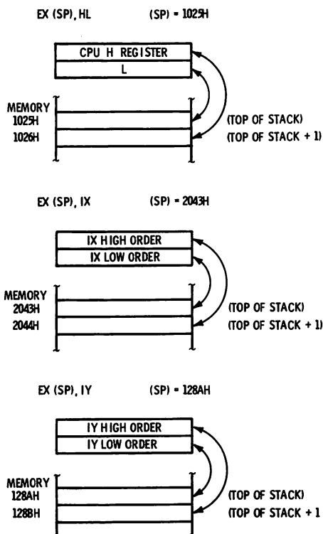
Fig. 5-5. EX (SP) instructions.
