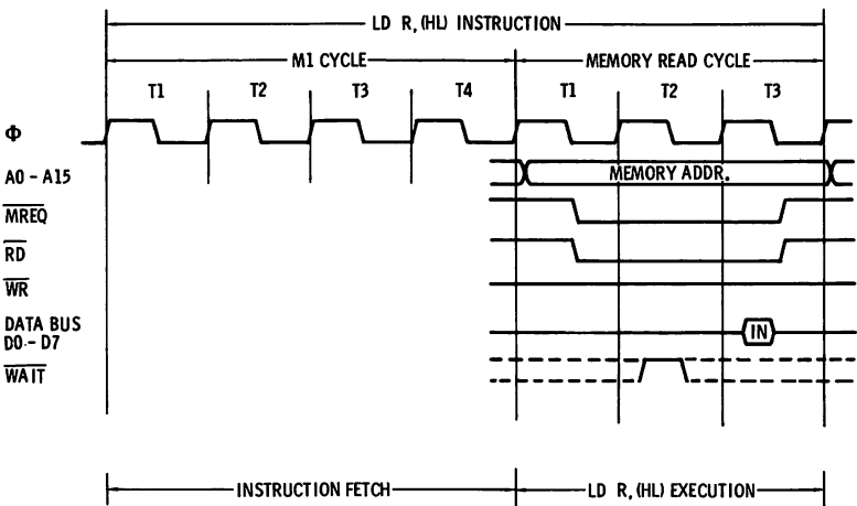
Fig. 3-4. Read cycle.
