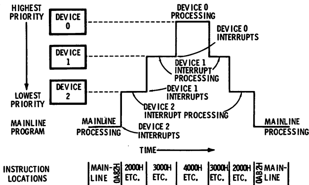
Fig. 7-8. Nested interrupt example.
