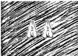
Listing 5
