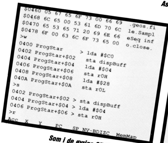
GeoProgrammer's Linker.
