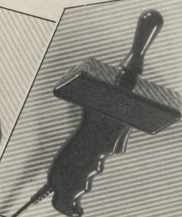
Phasor
