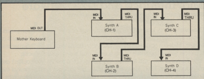
• Midi connections
