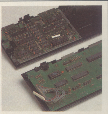
● Top: the new, lighter design: difficult to fix. Below, the old roomy circuit board
