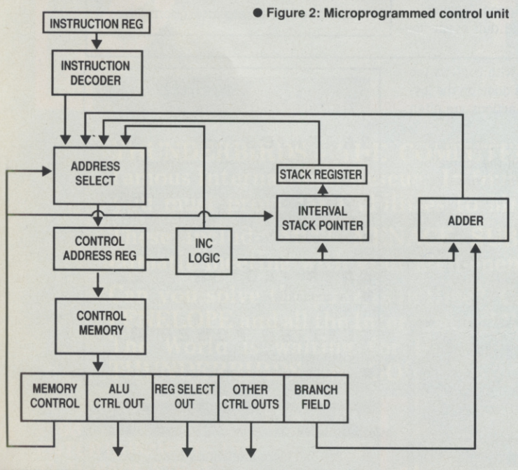
● Figure 2: Microprogrammed control unit
