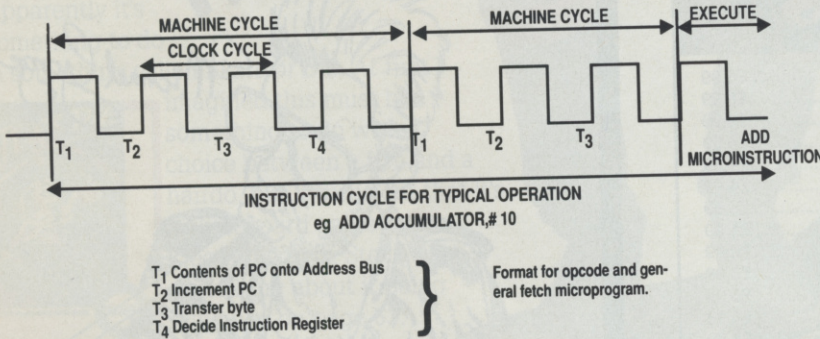
● Figure 3: an instruction cycle
