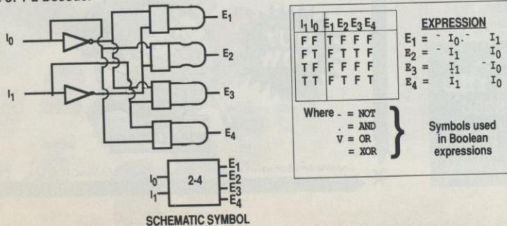
● Figure 5: 1-2 Decoder
