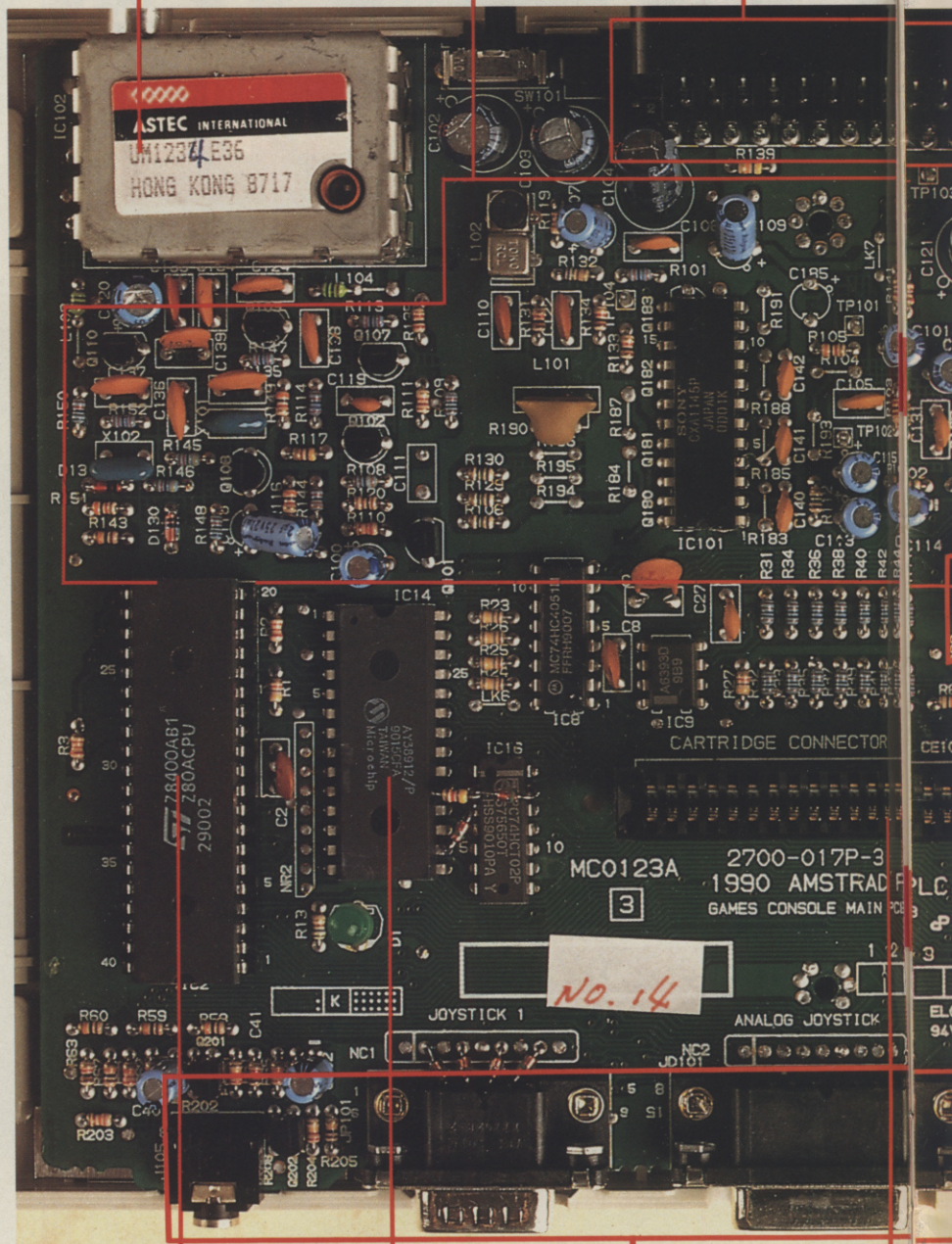
Sound Chip. The AY38912, as used in the original CPC range, provides three channels of sound.
