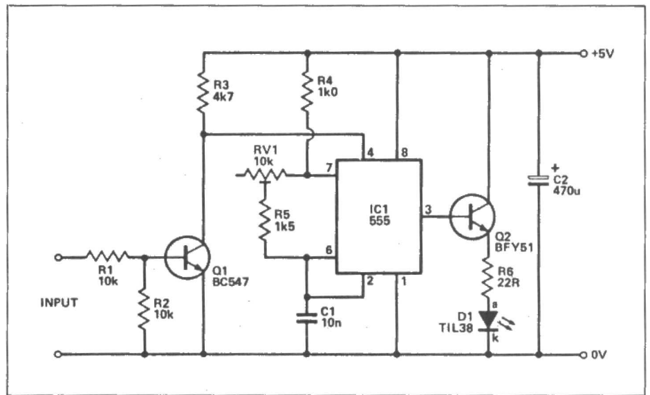
Figure 2. Circuit diagram of transmitter.
