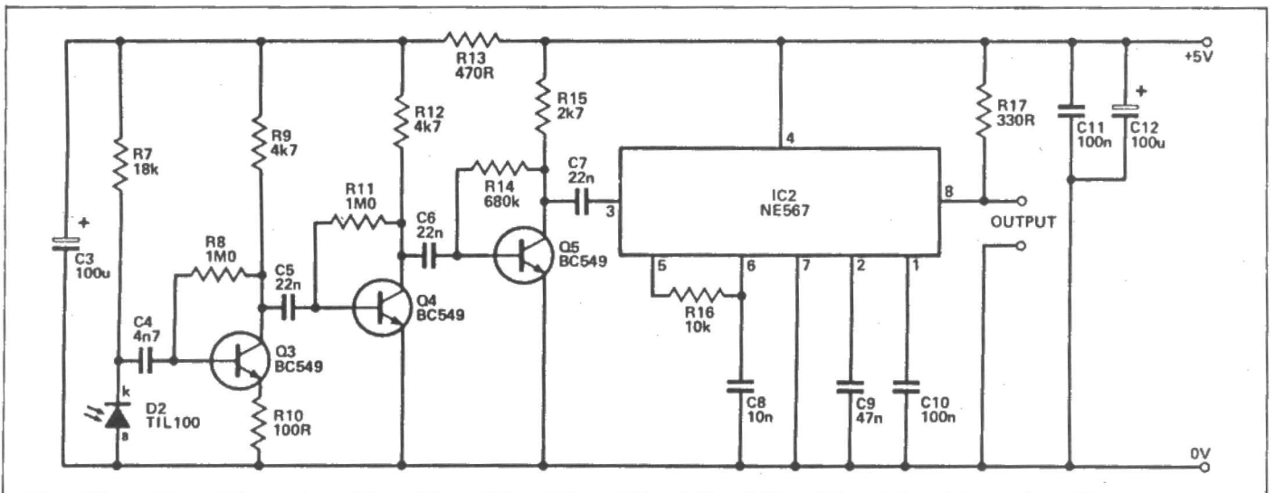
Figure 3. Circuit diagram of IR receiver.
