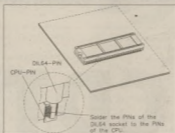
Each of the 64 legs of the DIL socket must be carefully soldered to the 68000 processor on the ST's motherboard.
