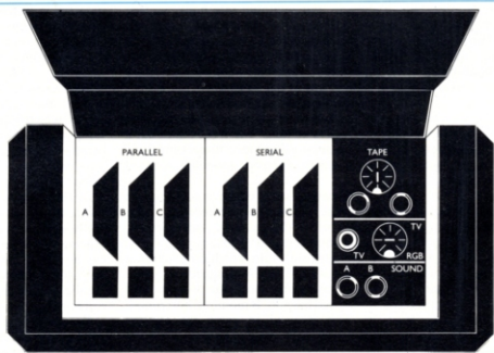
The rear hatch covers the main Input/Output connectors arranged in blocks. Parallel are at one end, serial in the centre, and the miscellaneous ones.
