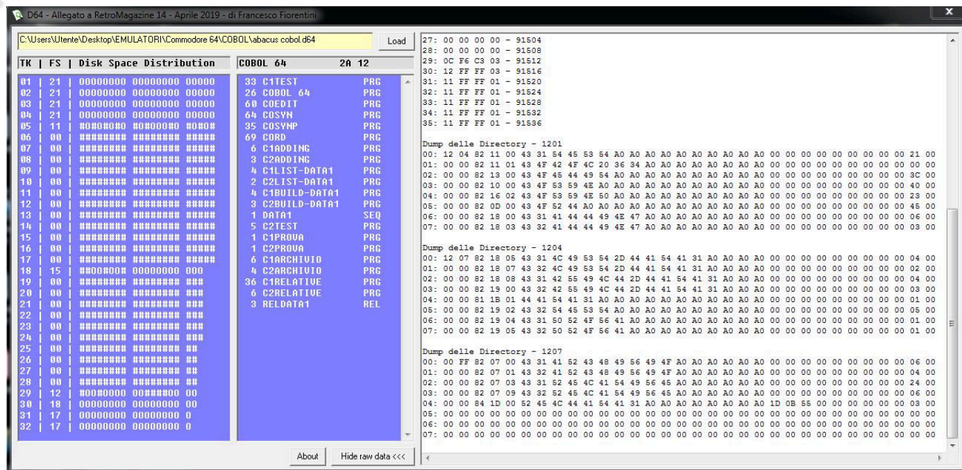
2. The Visual Basic 5 program coded to test the .D64 file format
