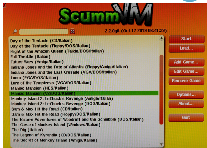
Figure 5 - ScummVM 2.2
