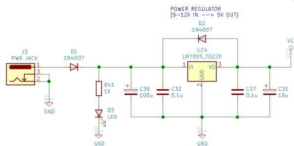
Figure 4: Circuit based on the LM7805
