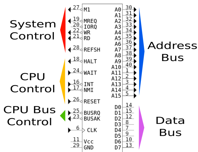
Figure 3: the pinout of the Zilog Z80 processor
