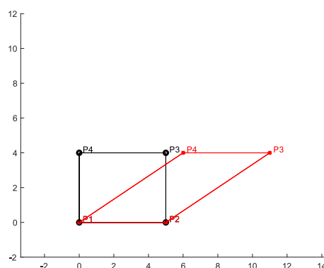
Figure 7. Shearing along the x -axis.
