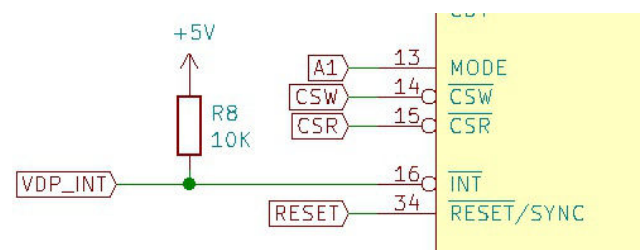
Figure 4: VDP pin "MODE"
