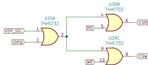
Figure 3: Logical ORs for selecting read and write signals for VDP
