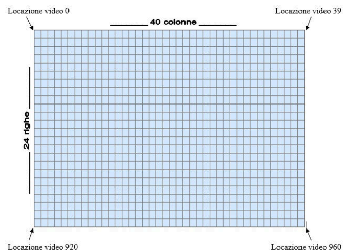
Fig. 3 - NAMES TABLE in the "MA1" mode
