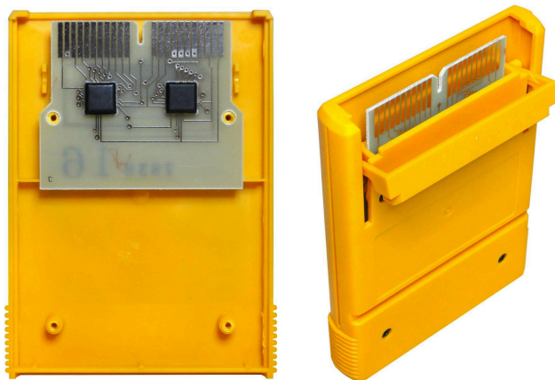
Fig. 4 - The inside of a Videocart and the contact protection flap (photo: Schnurrikowski- source: Wikimedia Commons)
