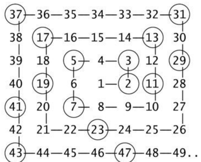
Fig. 1 - The Ulam spiral, was discovered by Polish mathematician Stanislaw Ulam in 1963, who noticed that prime numbers tended to align along the diagonals of the spiral.
