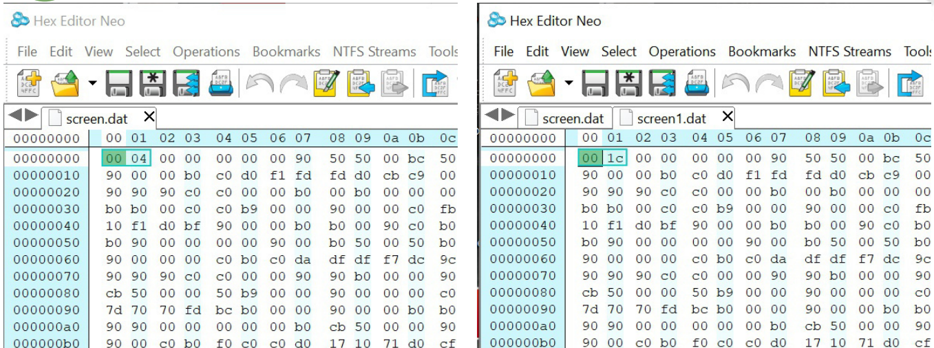
Fig. 3 e 4 - Screen C64 (left) and Screen C128 (right)
