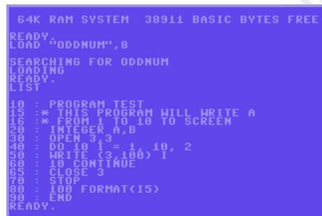
Fig. 4 - The program just typed in
