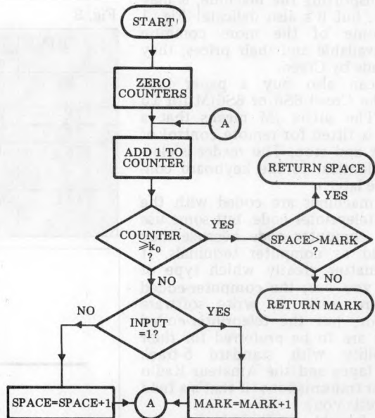
Subroutine BITCHECK
