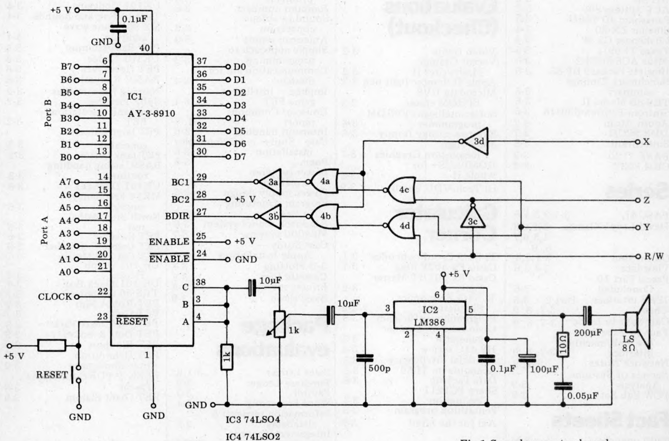
Fig 1 Sound generator board
