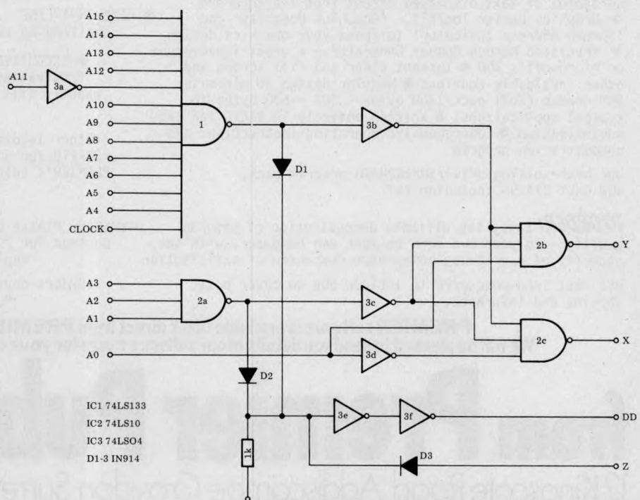
Fig 3 Address decoding. Point Z connects with the circuit of Fig 1 to pick up a R/W line.
