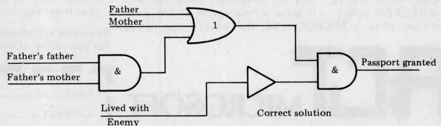
Fig 22 Better solution — fewer gates
