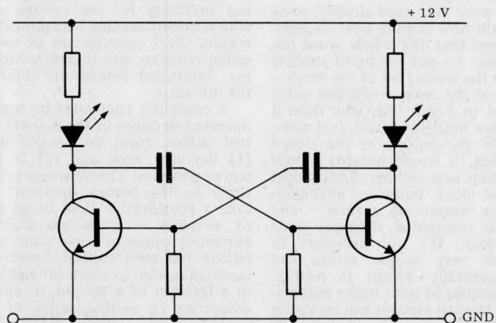
Fig 26 Astable
