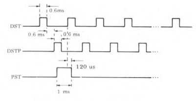
Fig 11 Timing signals
