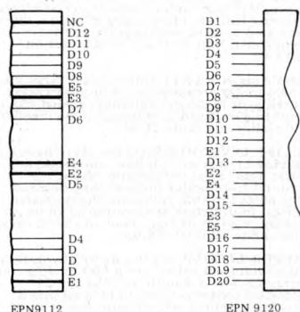
Fig 3 Connections to EPN printers.
