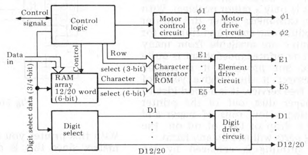
Fig 5 Block diagram of suggested control circuit for TI thermal printer units.
