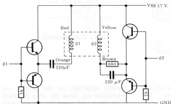
Fig 4 Suggested drive circuit and timing for stepping motor.
