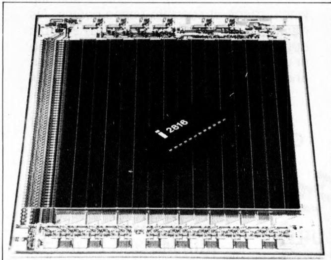
This is a picture of a hell of a lot of very special transistors. They are Intel's new electrically erasable permanent memory, the closest step so far to a memory chip that retains its memory when the power fails but functions normally. Putting data into this new 16 kbit chip (2 kbytes) takes absolute ages — a 21 volt pulse is needed for 10 milliseconds. A computer that had to store data at that speed would never get anything done, so clearly that side has a long way to go. But at least it is no longer necessary to pull the chip out of the computer and bake it under ultra-violet light to get rid of the data when it isn't wanted. Instead, it takes 20 milliseconds to erase eight bits with another electrical pulse.
