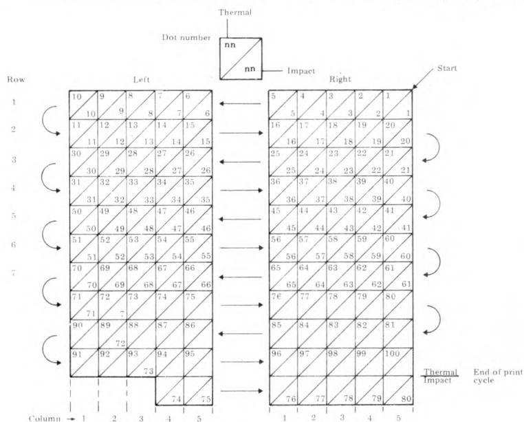
Fig 13 Character cells covered by print element.
