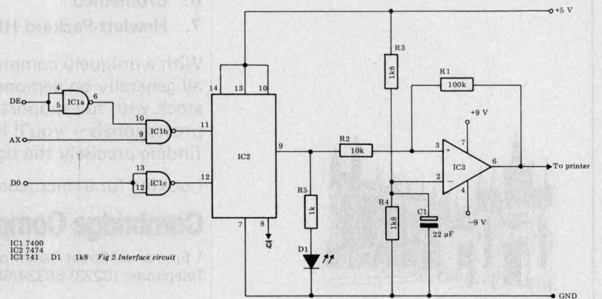
Fig 2 Interface circuit
