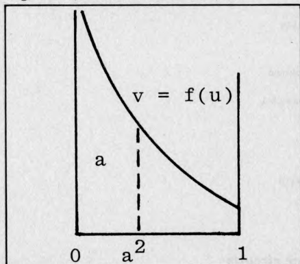
Fig 9 Distribution of X^2
