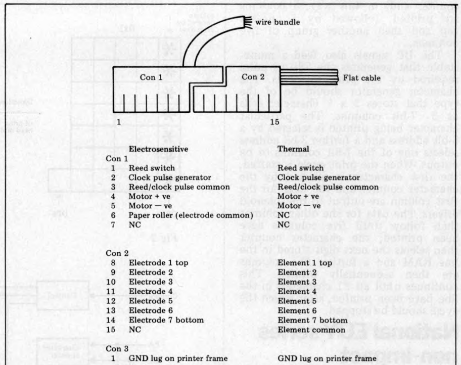
Fig 5 Connector pin-outs for EUY 10E/10T printers.
