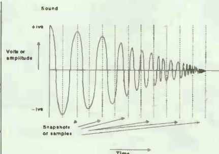
Fig 1 The frequency of the sound wave is increasing with time, yet the sample rate shown can only accurately record the first few wavelengths. The diagram also clearly shows that a sample is needed at both +ive and -ive peaks in order to record the wave's frequency correctly; therefore, the highest frequency that a sampler can record is half the sample rate.
