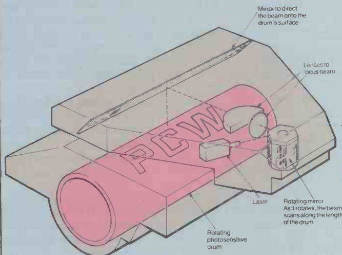
Expanded view of the drum and laser
