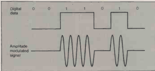
Fig 1 Amplitude modulation
