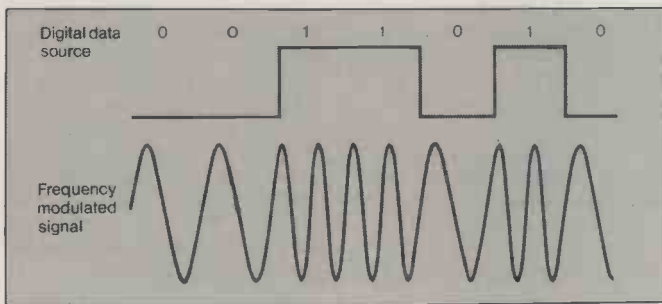
Fig 2 Frequency modulation
