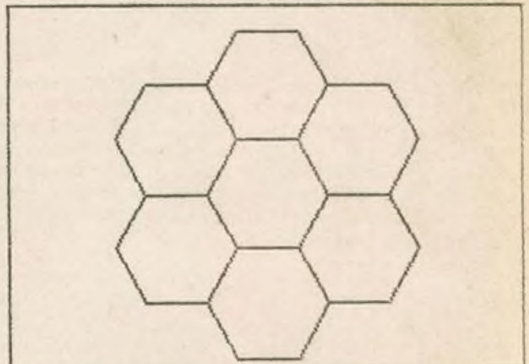
example 4 goto 113 110 0 daisy hex rep 6(dra 30 tur 60) daisy rep 6(hex mov 30 tur -60)
