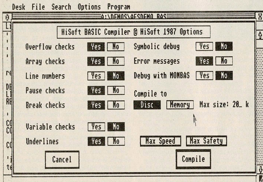
Compiler menu
