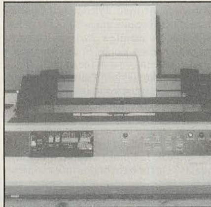
Bidirectional printing and motion minimisation are controlled by firmware. The print wheel carries an inner ring of characters.
