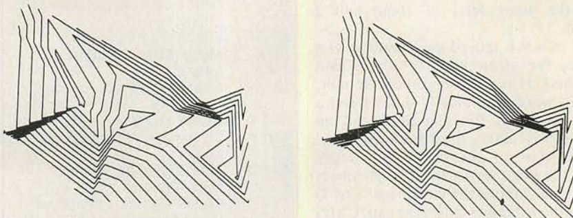
Figure 2. Stereogram of data set with hill shading and viewed from the side.
