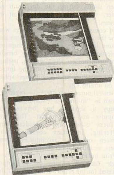
The Gould Colourwriter is a digital plotter which can add plotting to almost any computer system. It can use up to 10 pens. There is an integral buffer memory which is expandable from 2K to 16K and five character sets are included as standard.
