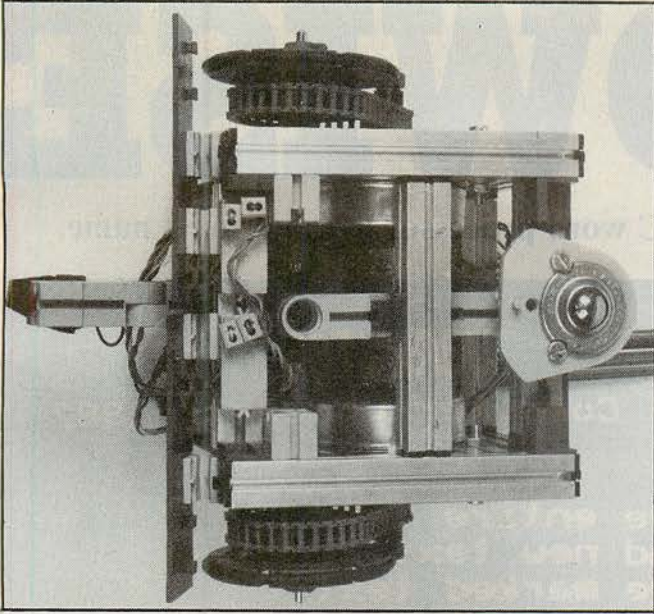
The wheels are driven independently by stepper motors.
