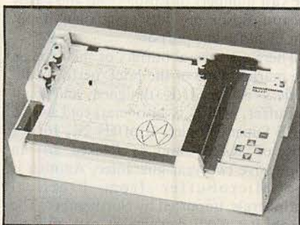
The Pixy 3 is a three-colour plotter aimed at the personal-computer user. Its own local intelligence comes courtesy of a Z-80 processor which helps in the generation of circles, arcs and curves. There are nine character sets plus scientific symbols, nine line types with a variable pitch and 15 character sizes. Pixy 3 costs £599 from Mannesmann Tally.
