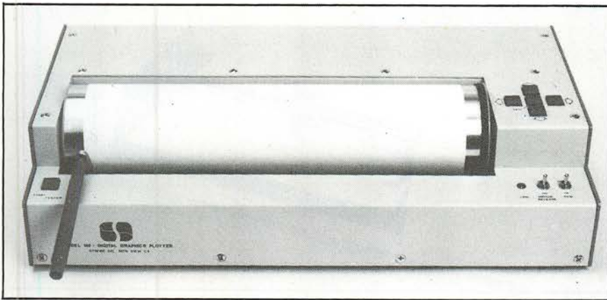
The Strobe 100 drum plotter from Data Efficiency comes complete with BBC software.
