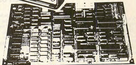
The heart of the system — MICRONIX 80HD Single Board Micro — also available separately.
