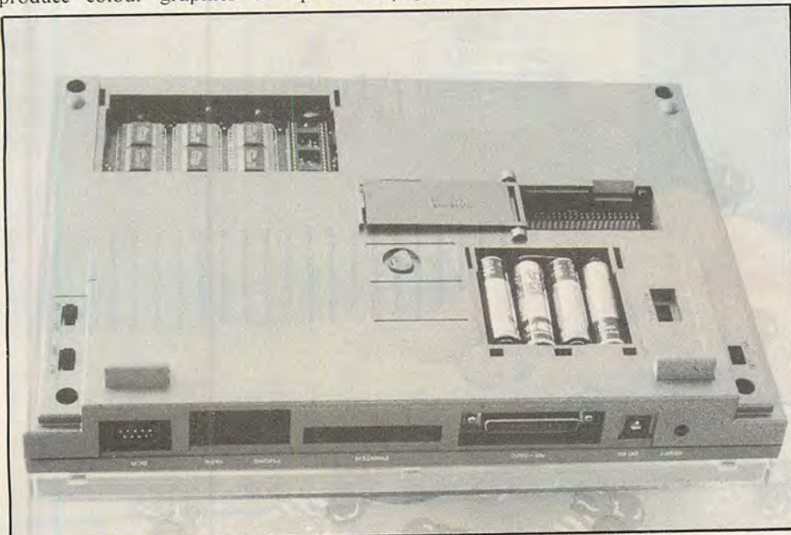
Expansion ROM and RAM sockets, bus connector and batteries are in the base.
