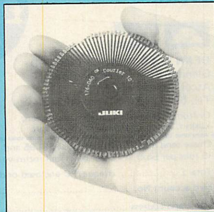
A typical daisywheel has 96 characters mounted on the end of flexible stems.
