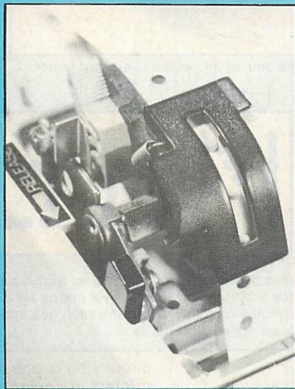
In a tractor-feed mechanism a pair of notched wheels engage in holes punched down each side of the paper.
