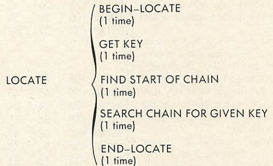
FIGURE 1. WARNIER DIAGRAM OF THE PROBLEM.
