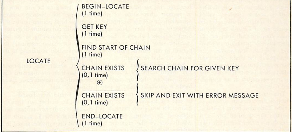
FIGURE 2. INCORPORATING EXPANSION OF CHAIN EXISTS STATEMENT.
