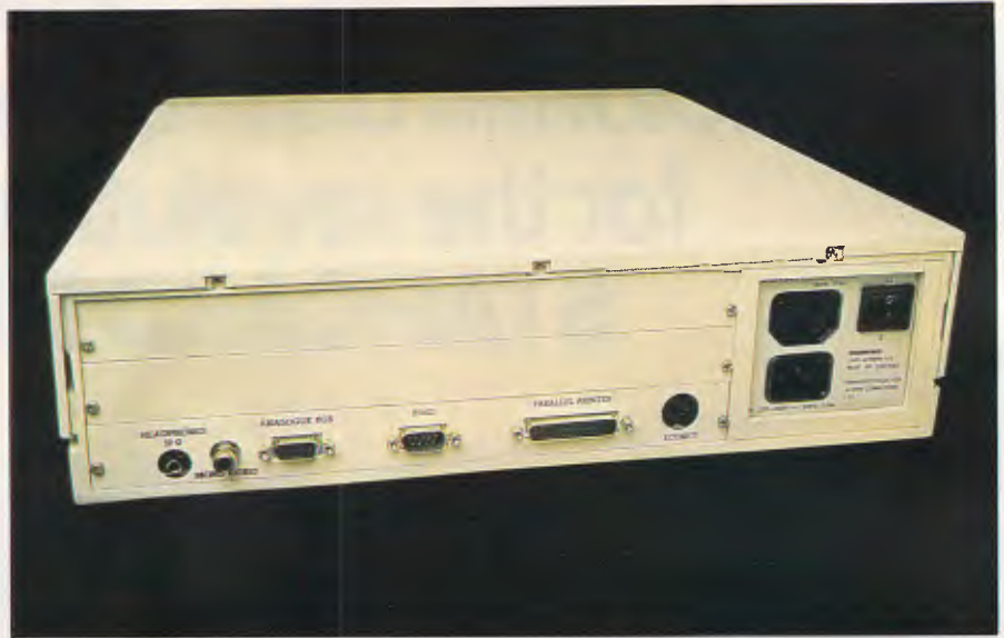
The back of the Archimedes is relatively sparse by today's standards, consisting of: headphone sockets, mono video out, analogue RGB, serial, parallel and Econet. The two removable plates above the ports will accommodate 'podules' — that is, peripheral modules
