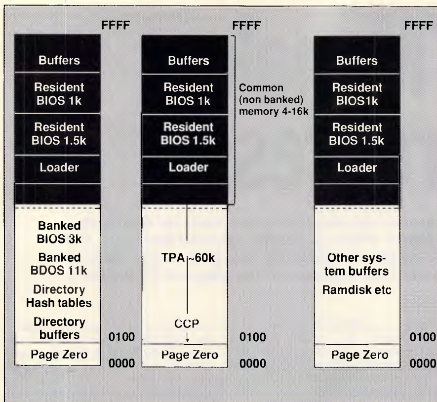
Fig 1 Memory map of banked CP/M Plus system
