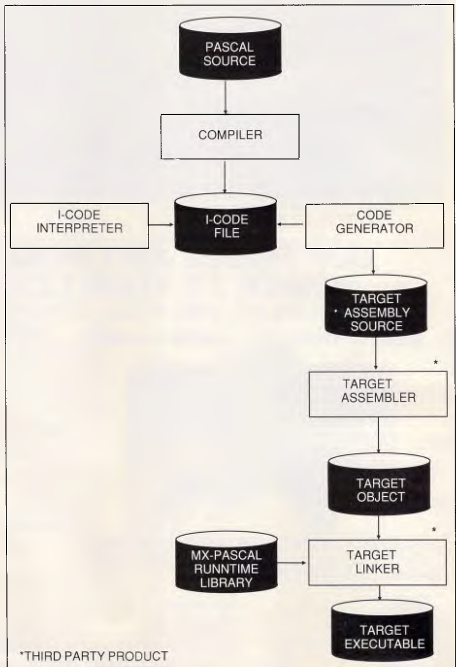
Figure 1 Structure of MX-PASCAL
