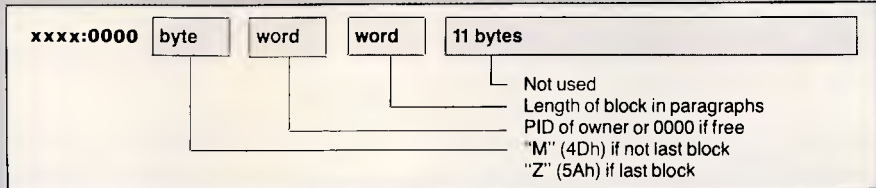
Fig 1 The structure of a DOS Memory Control Block
