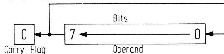
Abb. 3 RLC
