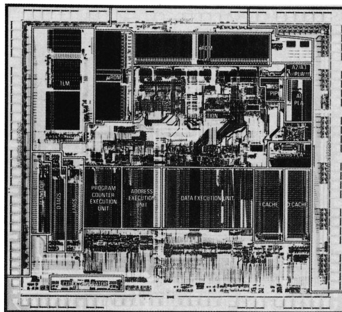
Motorola's MC68030
