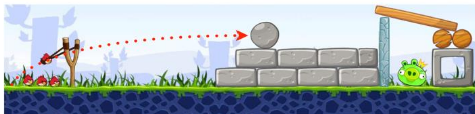
Figura 1 Angry Birds
