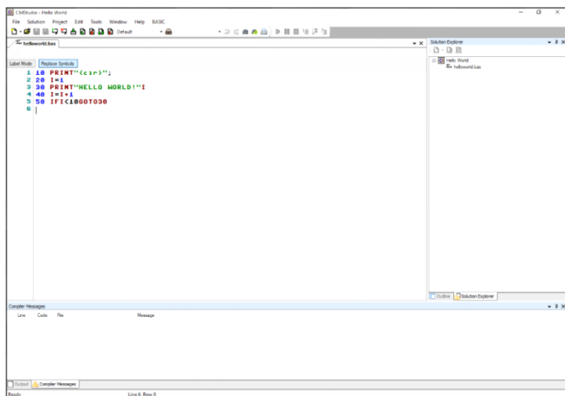
Fig. 3 – C64 Studio
