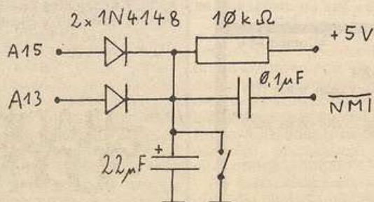
Skica 2: restart 5FFFH
